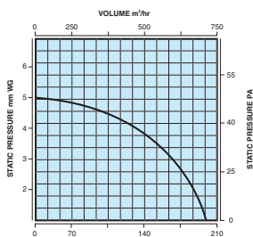
Performance Graph WF230 Series 668m 3 /hr 185 litres per second
