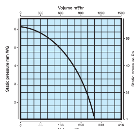
Performance Graph WF300 Series 1100m 3 /hr, 306 litres per second
